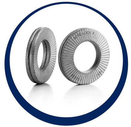
NORD LOCK WASHER
